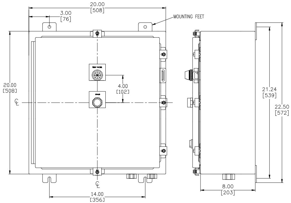
BBS-60500-(SERIAL NUMBER) BBS BATTERY AND CONTROL UNIT
