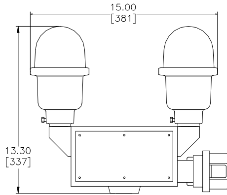
POL-21003-R-3F-34B-DT-P TYPICAL 12VDC POL WITH OPTION -P
